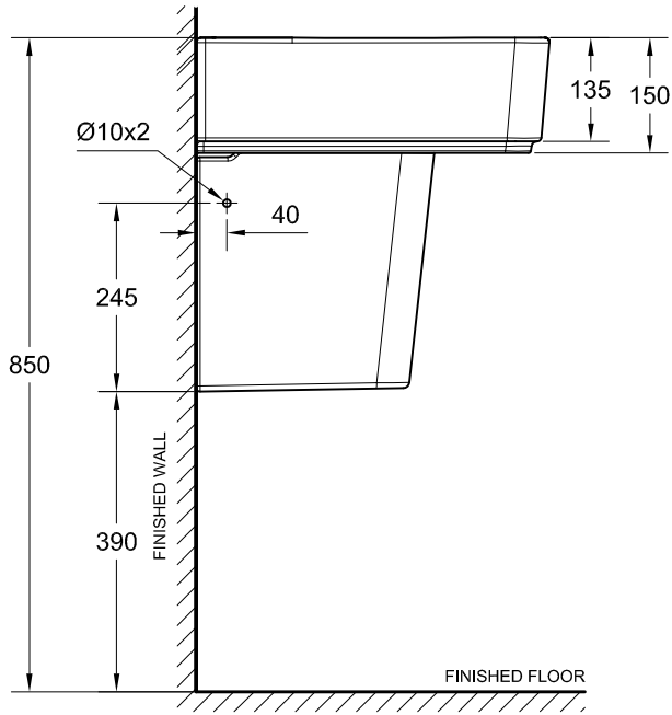
SIDE VIEW
